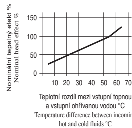
Korekce teplot, Correction Temperature teplota, Temperature, diagram A
